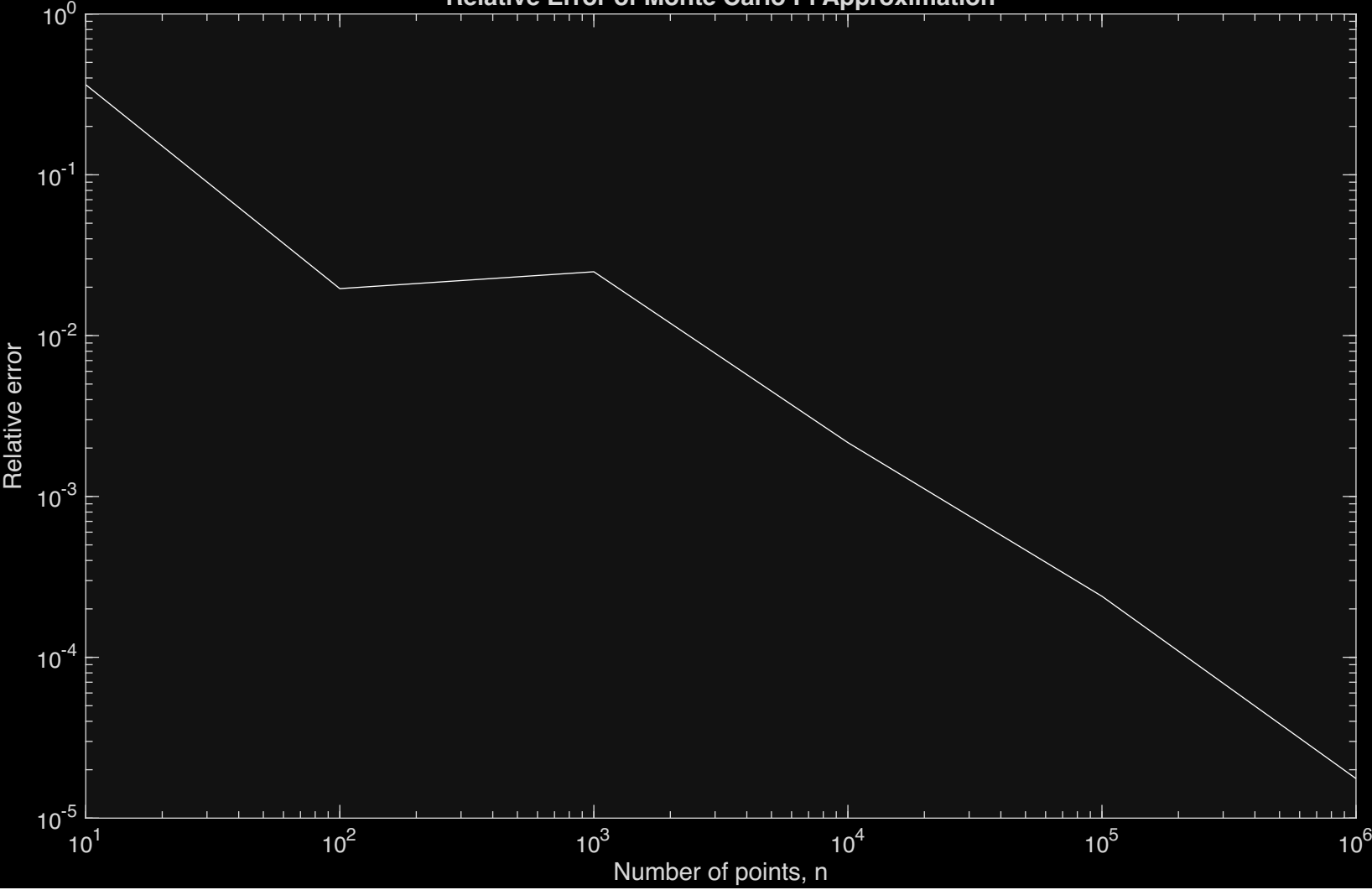
Relative Error of Monte Carlo Pi Approximation
